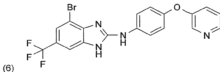
(4-Brom-6-trifluormethyl-1H-benzimidazol-2-yl)-[4-(pyridin-3-yloxy)-phenyl]-amin
